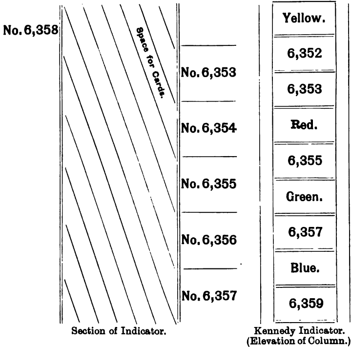
FIG. 67.—Diagrams of Kennedy Indicator (Section 208).
